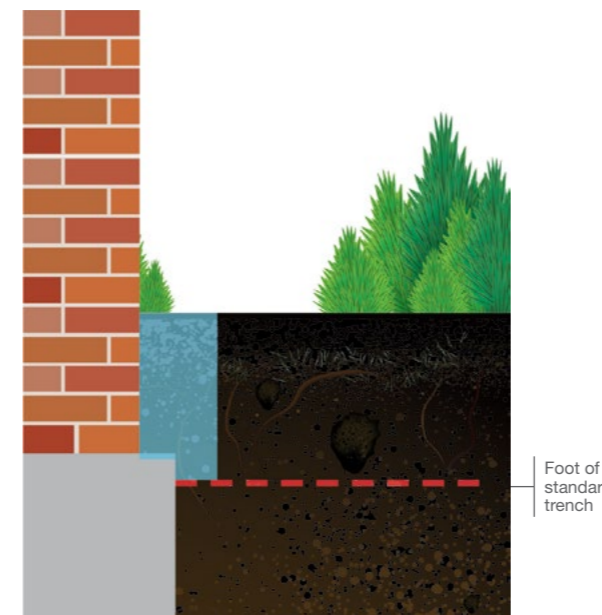
Conventional treatments require significant trenches to be excavated well below the footing. The trenches are then backfilled with treated soil to form the protective zone. This large scale excavation can lead to significant disruption and damage to landscaped areas.
