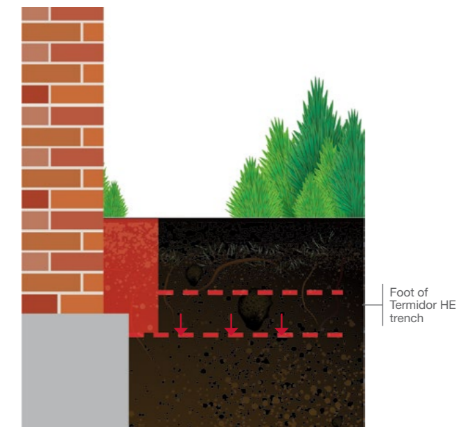
Termidor HE is applied in shallower trenches. Advanced polymer technology then allows its active ingredient to spread down and form a protective zone that is at least as deep as standard treatments provide. This results in a superior treatment with less disruption and damage.
